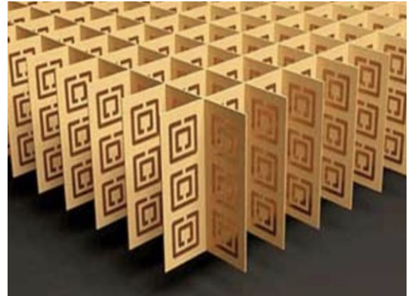
Figure 1. Metamaterial lattice is used to demonstrate negative refraction. The array of square split-ring resonators gives the material a negative magnetic permeability, whereas the array of straight wires gives it a negative permittivity. (Source: Houck, Andrew A.; Brock, Jeffrey B.; Chuang, Isaac L. "Experimental observations of a left-handed material that obeys Snell's law". Phys. Rev. Lett. American Physical Society.)
