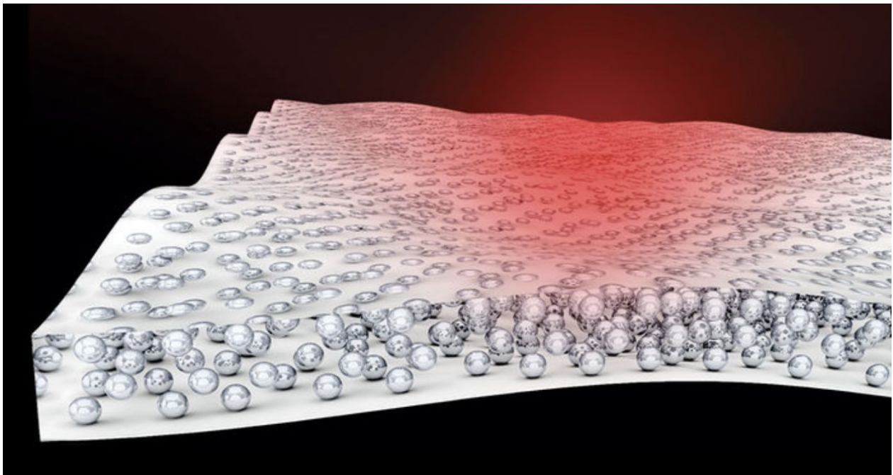
Figure 3. Radi-Cool technology uses ~10 \mu\text{m} in diameter glass spheres, embedded in a flexible polymer to create a thin-film cooling material. (Courtesy of Radi-cool)
